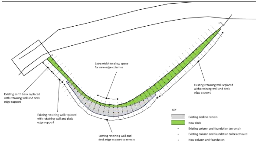
Figure 14: Illustration of extension to stilt structure supporting the Longbridge SLTL
