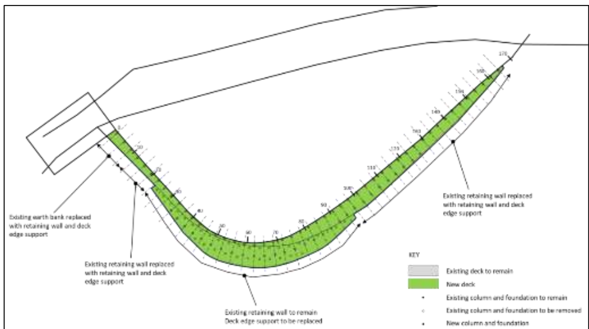
Figure 15: Illustration of proposed stilt structure supporting the Longbridge SLTL.
