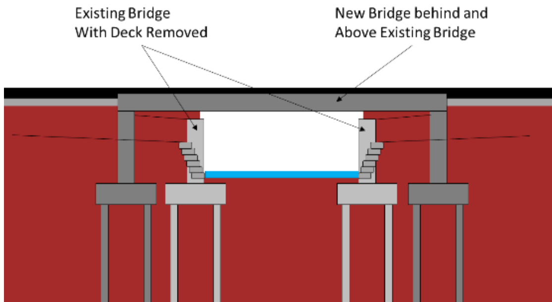
Figure 12: Illustration of assumed new A23 Brighton Road Bridge
