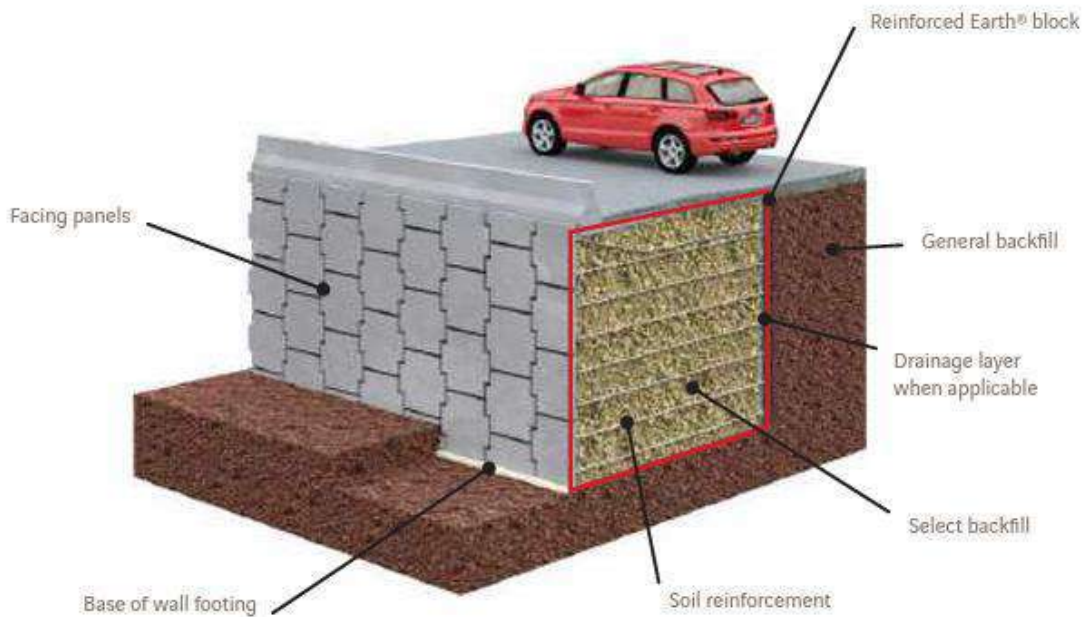
Figure 25: Typical reinforced earth-retaining structure 2
