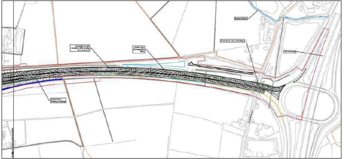
Figure 7: M23 Spur Improvements
