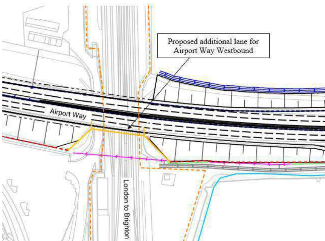
Figure 22: Airport Way Bridge Widening
