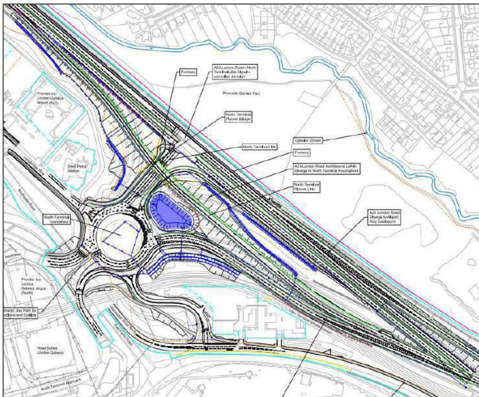
Figure 4: North Terminal Roundabout Improvements
